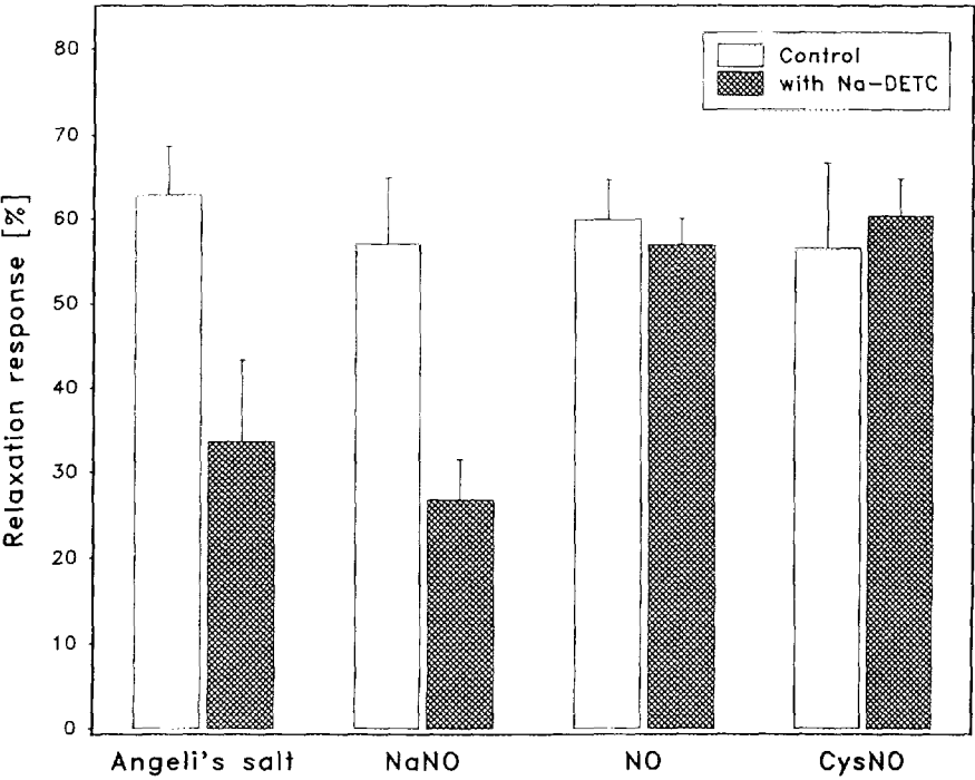
Fig. 3. Inhibitory effect of Na-DETC (0.1 mM) on the relaxation response to Angeli's salt (0.3 \mu M), NaNO (10 \mu M), NO \cdot (3 \mu M) and to CysNO (0.3 \mu M). Results are means \pm S.E.M. of 3 experiments.
